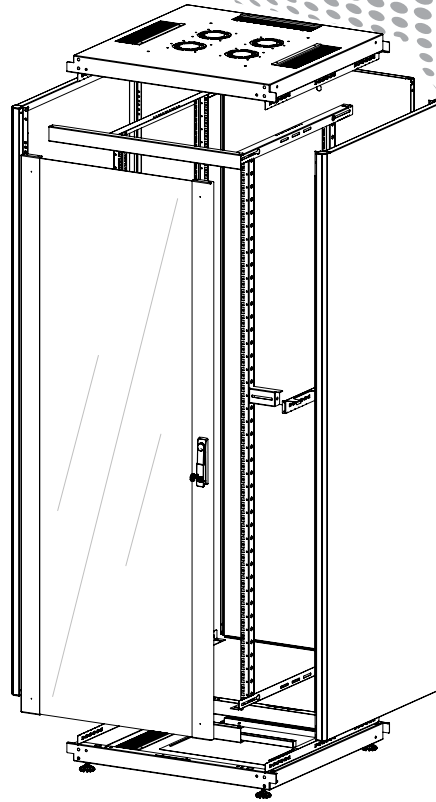
EXPLODED VIEW
