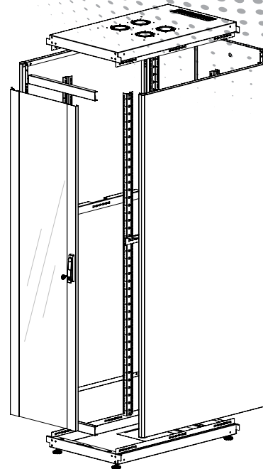
EXPLODED VIEW
