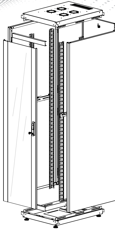
EXPLODED VIEW
