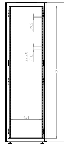
DIMENSIONS IN WIDTH AND HEIGHT
