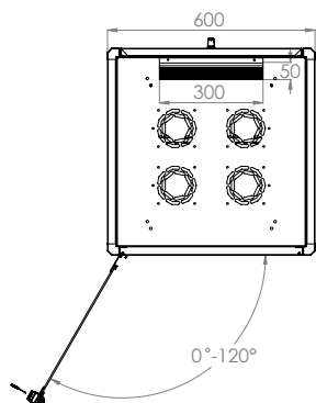
FRONT DOOR OPENING ANGLE
