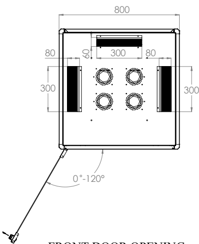
FRONT DOOR OPENING ANGLE
