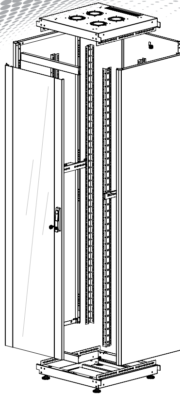
EXPLODED VIEW
