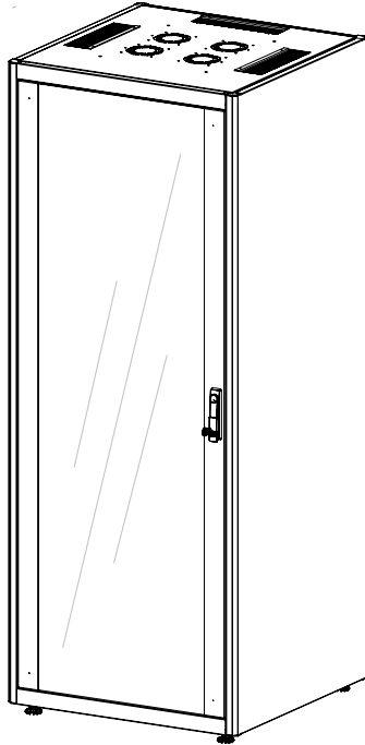
ISOMETRIC VIEW
