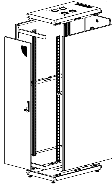
EXPLODED VIEW
